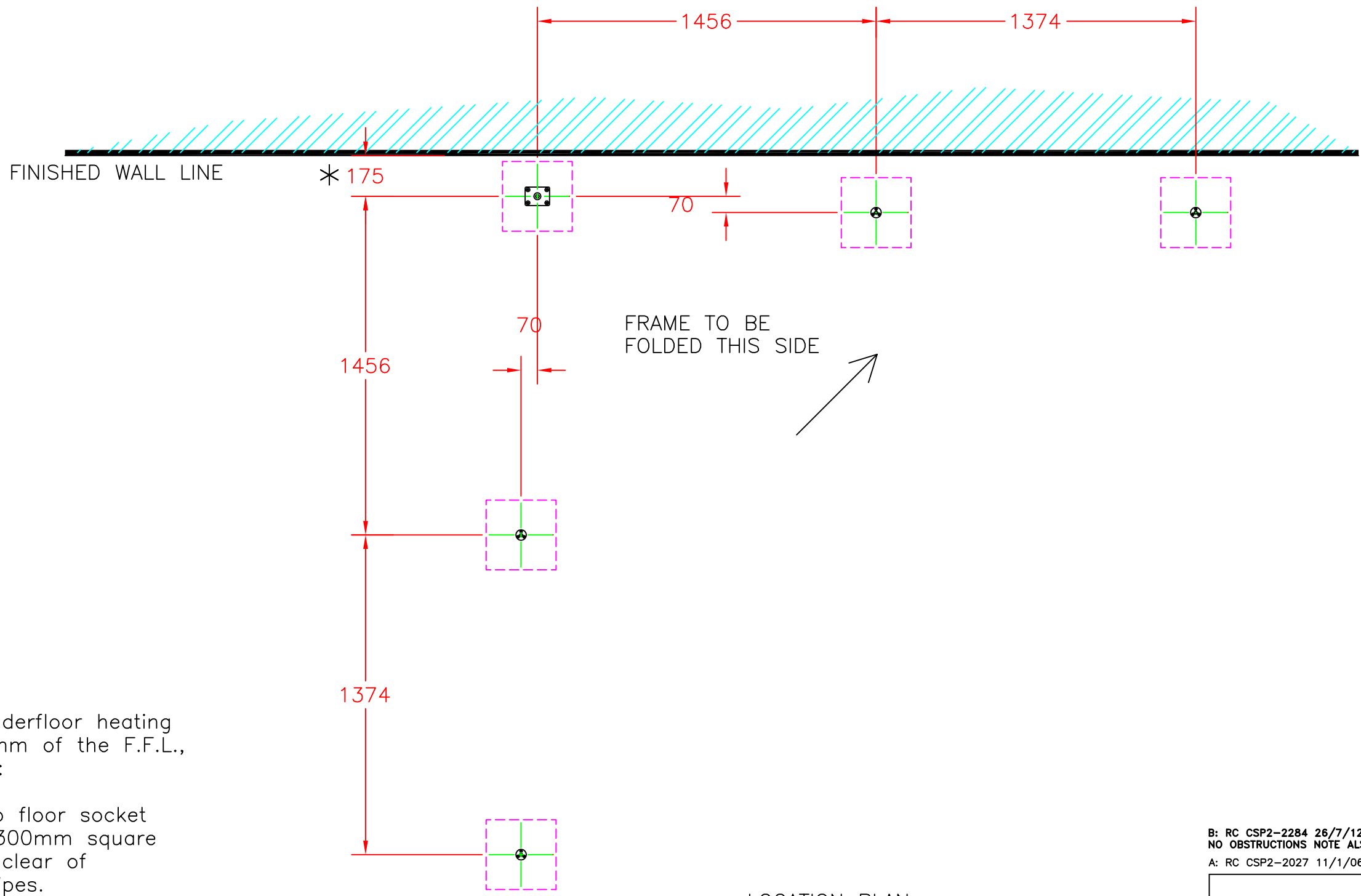
LOCATION PLAN
