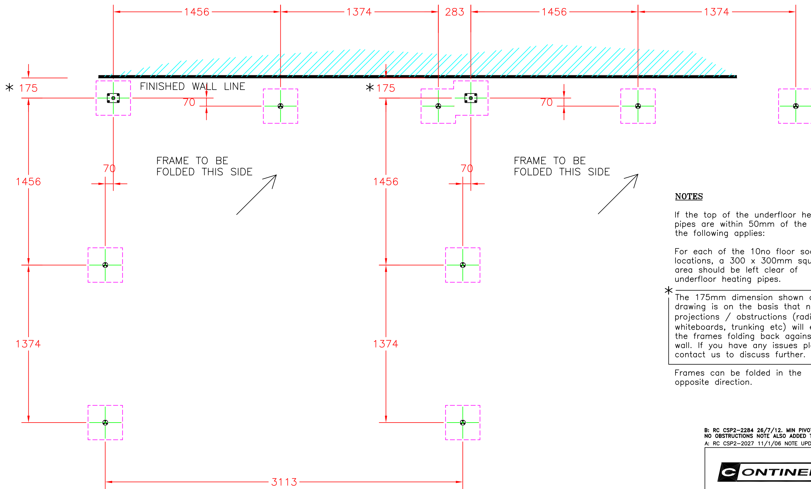
LOCATION PLAN
