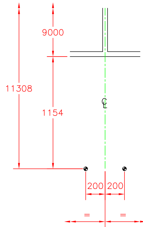
INTERNATIONAL MODEL VOLLEYBALL POSTS (SCALE 1:20)
