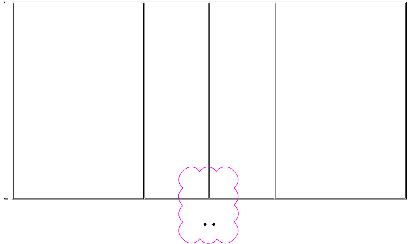
INTERNATIONAL MODEL VOLLEYBALL POSTS (SCALE 1:20)
